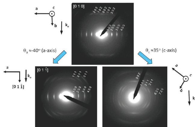
Figure 3. Rotation-tilt experiment performed on an oriented P3HT film (7.9 kDa) grown by slow-rate directional crystallization in TCB. The sample shows initially a (0 1 0) contact plane ([0 1 0] zone). A tilt around the a axis by \sim 40^\circ yields the ED pattern typical of the [0 1 -1] zone with some contribution from the [0 1 1] zone. A tilt of the sample around the c axis by 35^\circ yields an ED pattern corresponding to the superposition of the [-1\ k\ 0] zones with k = 1, 2 , and 3.
